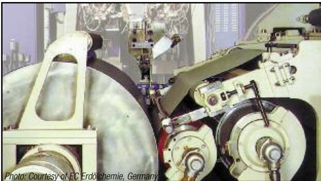
Monitoring edge temperature with EC150 reduces scrap and ensures proper film temperatures for strong film-to-paper adhesion.
